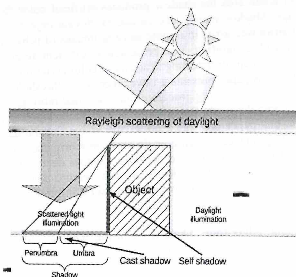
Figure 1. Shadow area formation.
